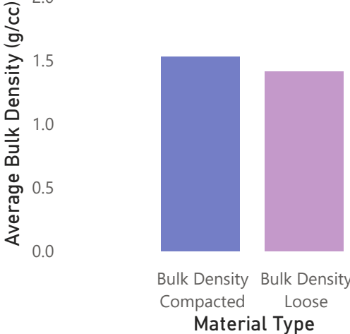
Average Bulk Density by Test Type (g/cc)
